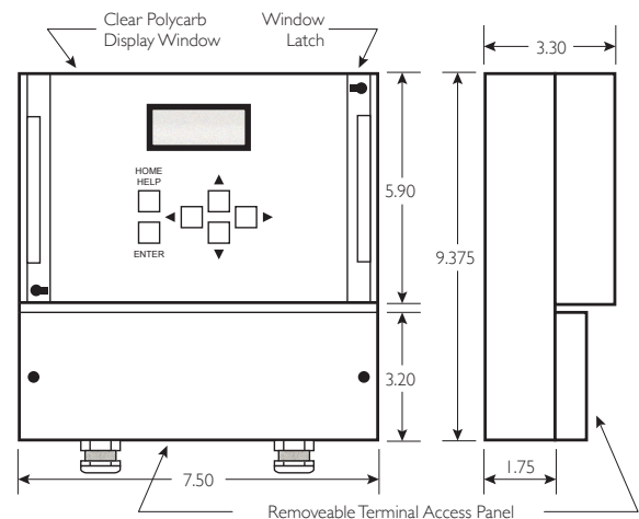
Monitor Dimensions
